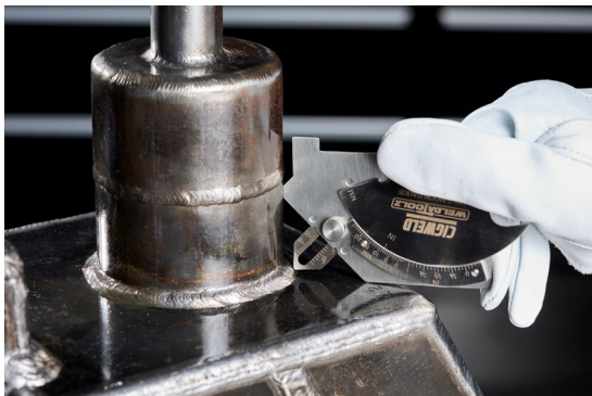
Half moon - Throat Size
