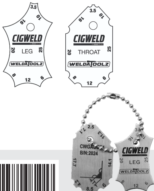
2-PCE Fillet Gauge P/N: CWGAUGE1
