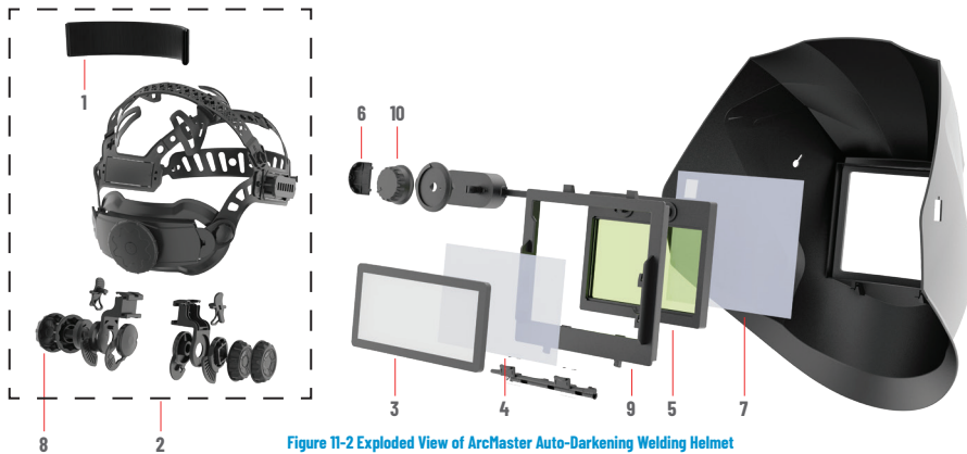
Figure 11-2 Exploded View of ArcMaster Auto-Darkening Welding Helmet
