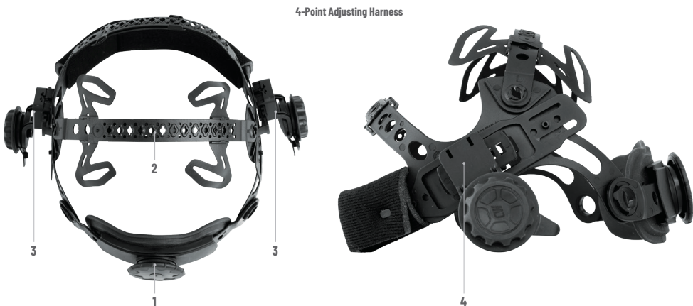
Figure 6-1 Harness Adjustment
