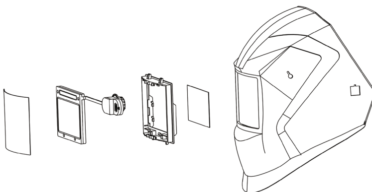
Figure 8-1 Exploded Line Drawing of Arcmaster Front & Rear Lens Positioning
