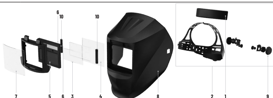
Figure 11-1 Exploded View of ArcMaster Auto-Darkening Welding Helmet
