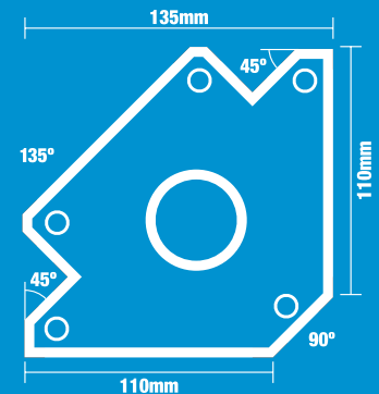
Large Clamp Holder Dimensions
