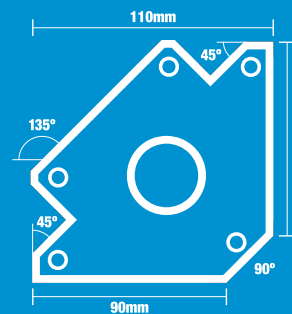
Medium Clamp Holder Dimensions
